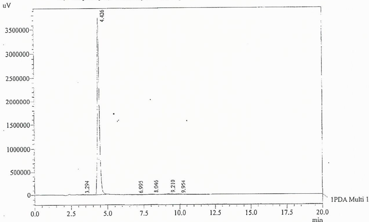
Chromatogram 2',4'-Dihydroxy-3,4-Dimethoxychalcone D:\promonence\Data
